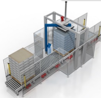
PF 40 ROTATING ARM
